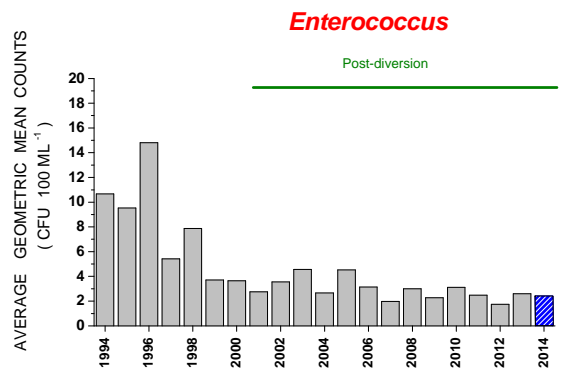
Fig. 17. Average Enterococcus counts by year, 1994-2014.
