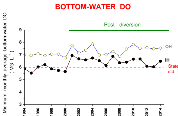
Fig. 15. Minimum monthly average bottom-water DO concentrations in IH and OH.
