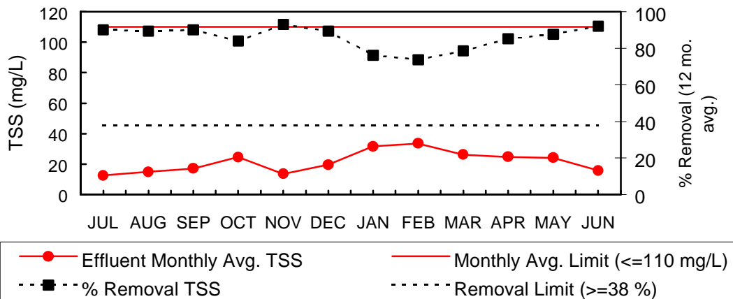
Figure II.B.2 Deer Island Treatment Plant Effluent TSS Trend Analysis, FY99
